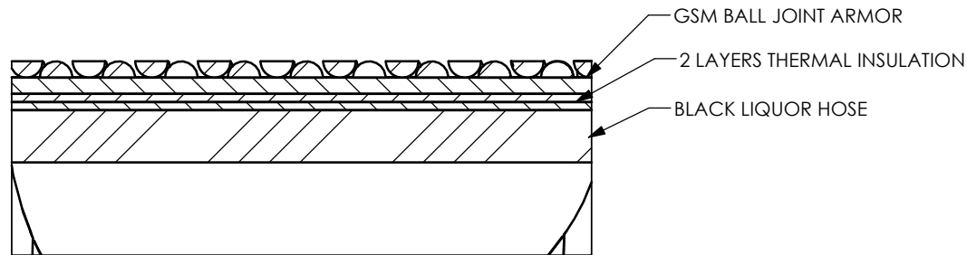
DETAIL A SCALE 1.5 : 1
