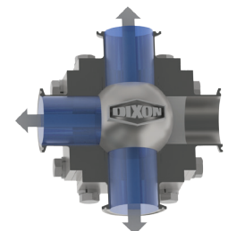
4-way 'T'-port position D
