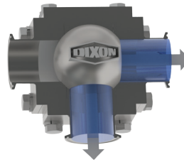
3-way 'L'-port position B
